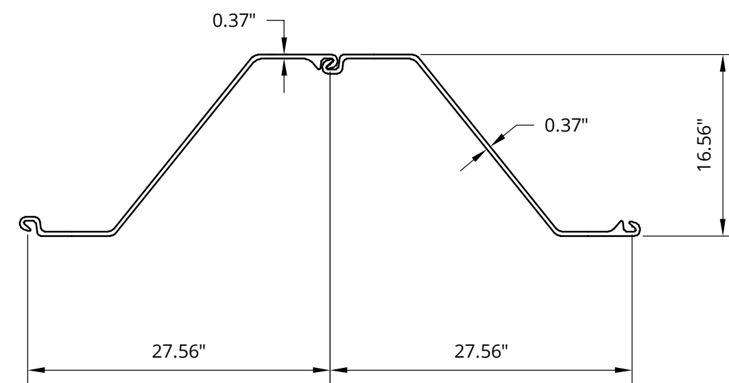
SHEET PILE RETAINING WALL SECTION - SKYLINE STEEL AZ 19-700
