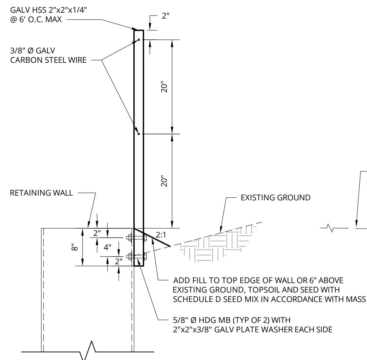
SECTION
