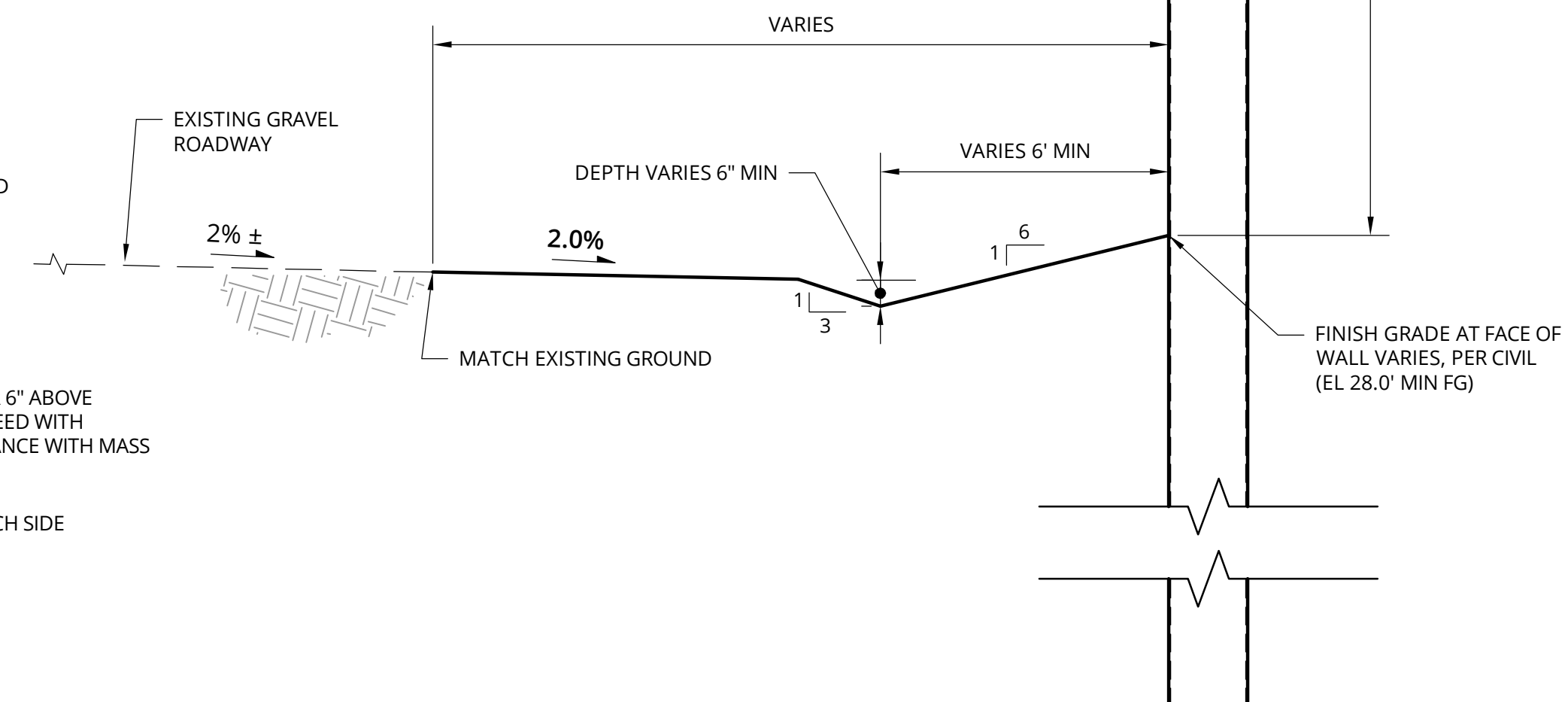
TYPICAL RETAINING WALL SECTION
