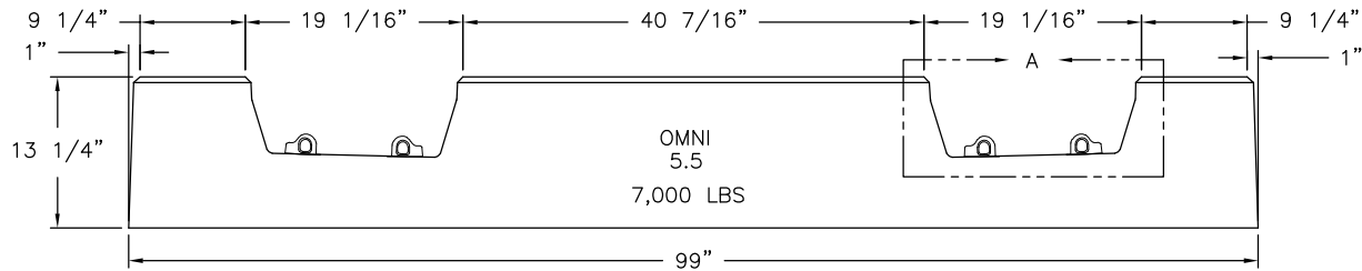
END VIEW
